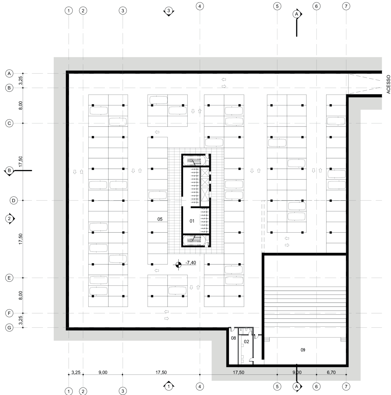
1 SUBSOLO 1:500
